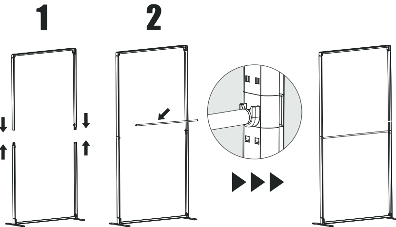
Basic frame
