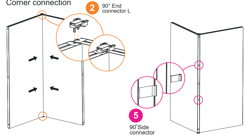
Corner connection
