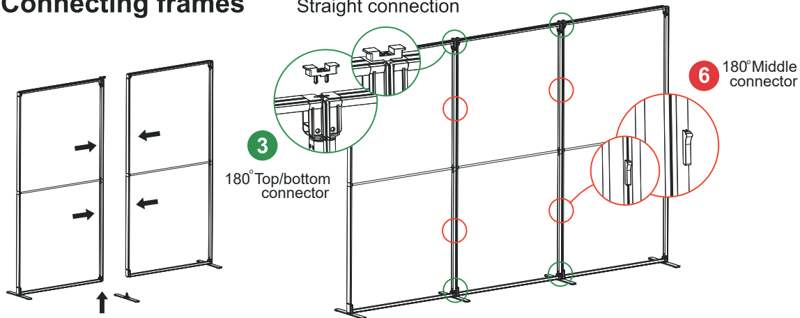
Straight connection
